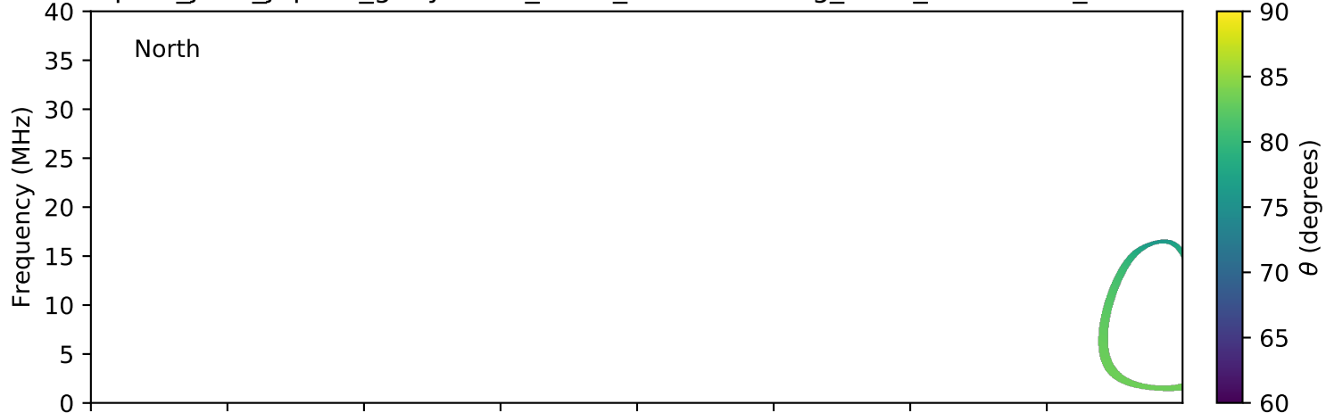
expres_juno_jupiter_ganymede_isaac_lossc-wid1deg_3kev_20160530_v01.cdf
