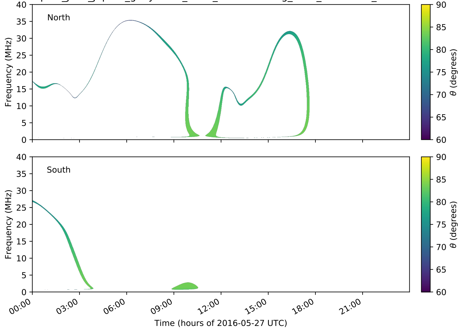
expres_juno_jupiter_ganymede_isaac_lossc-wid1deg_3kev_20160527_v01.cdf
