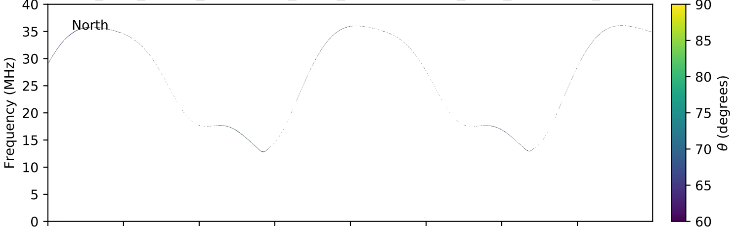
expres_juno_jupiter_ganymede_isaac_lossc-wid1deg_3kev_20160525_v01.cdf
