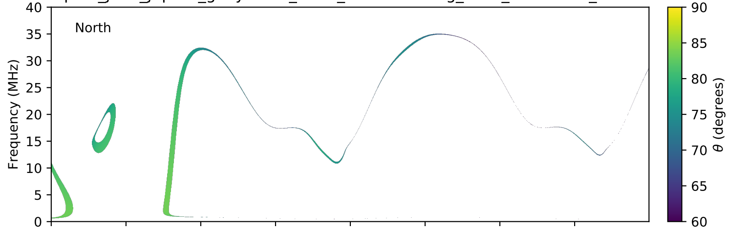
expres_juno_jupiter_ganymede_isaac_lossc-wid1deg_3kev_20160524_v01.cdf
