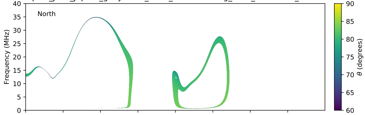
expres_juno_jupiter_ganymede_isaac_lossc-wid1deg_3kev_20160520_v01.cdf
