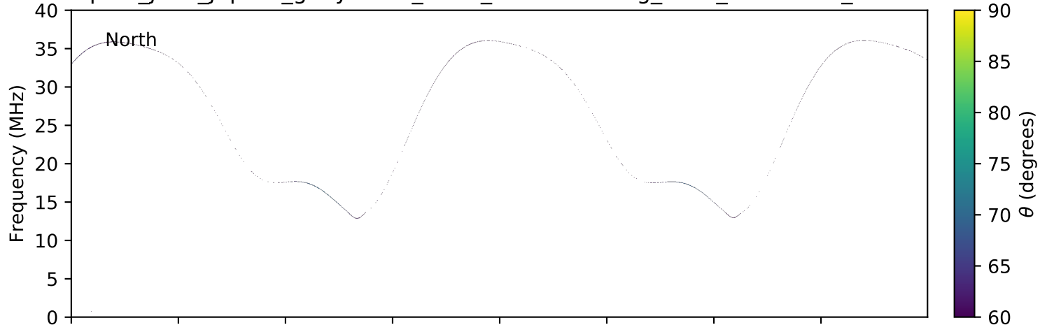
expres_juno_jupiter_ganymede_isaac_lossc-wid1deg_3kev_20160518_v01.cdf
