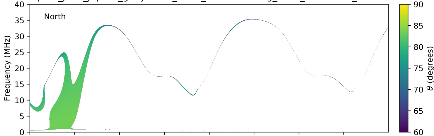
expres_juno_jupiter_ganymede_isaac_lossc-wid1deg_3kev_20160517_v01.cdf
