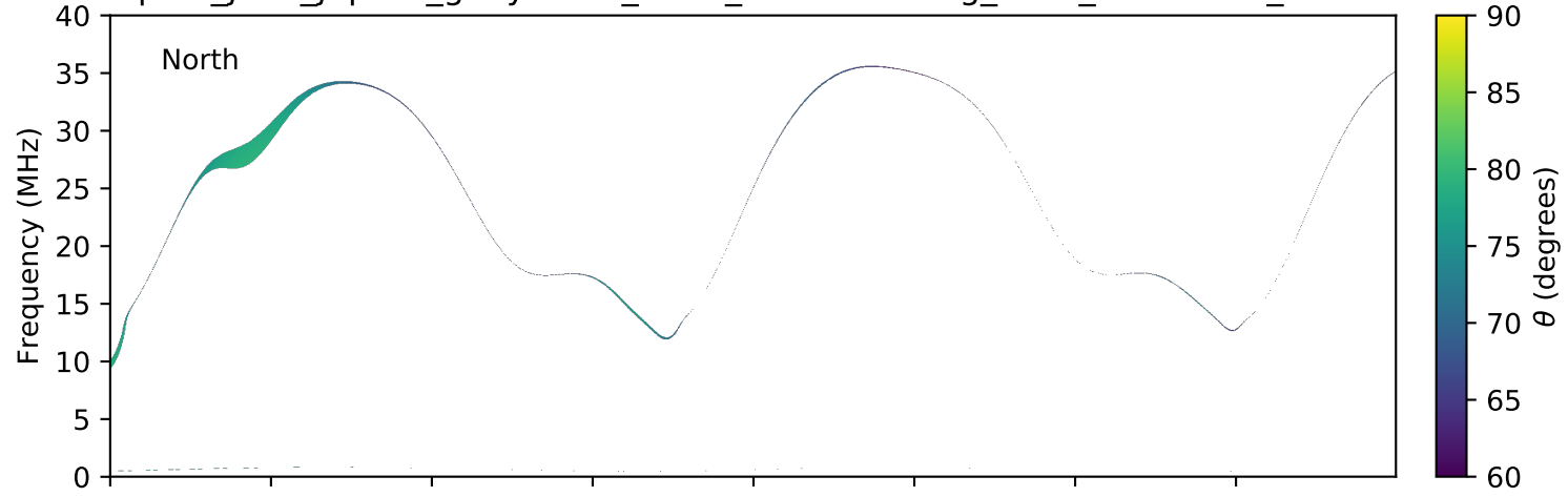
expres_juno_jupiter_ganymede_isaac_lossc-wid1deg_3kev_20160510_v01.cdf
