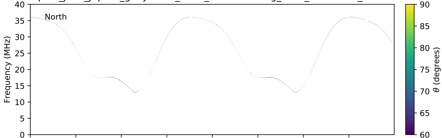
expres_juno_jupiter_ganymede_isaac_lossc-wid1deg_3kev_20160504_v01.cdf
