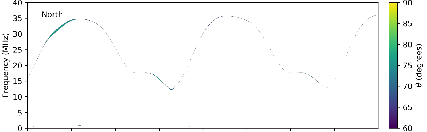
expres_juno_jupiter_ganymede_isaac_lossc-wid1deg_3kev_20160503_v01.cdf
