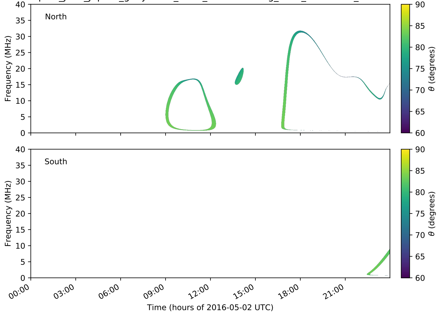
expres_juno_jupiter_ganymede_isaac_lossc-wid1deg_3kev_20160502_v01.cdf
