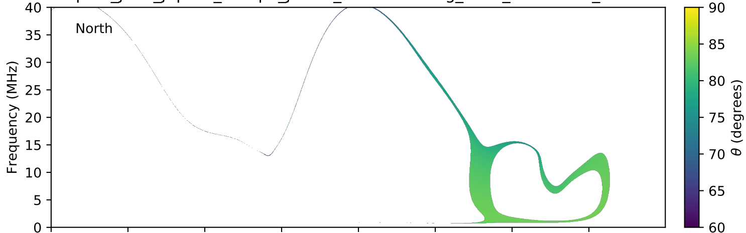
expres_juno_jupiter_europa_jrm09_lossc-wid1deg_3kev_20160528_v01.cdf
