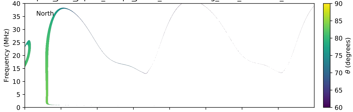
expres_juno_jupiter_europa_jrm09_lossc-wid1deg_3kev_20160527_v01.cdf
