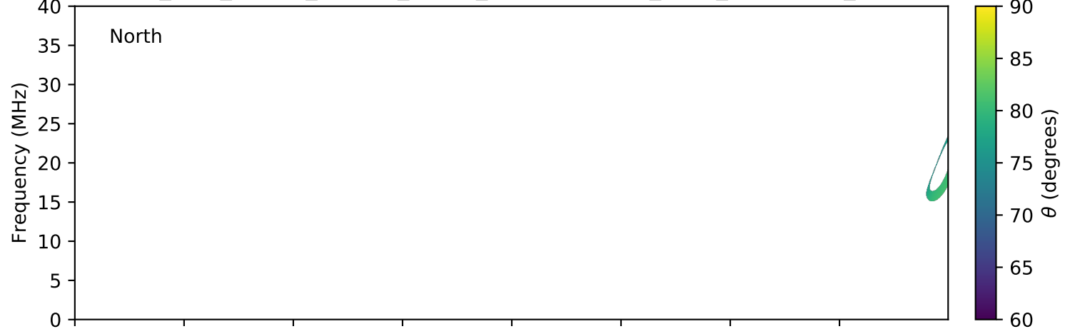
expres_juno_jupiter_europa_jrm09_lossc-wid1deg_3kev_20160526_v01.cdf
