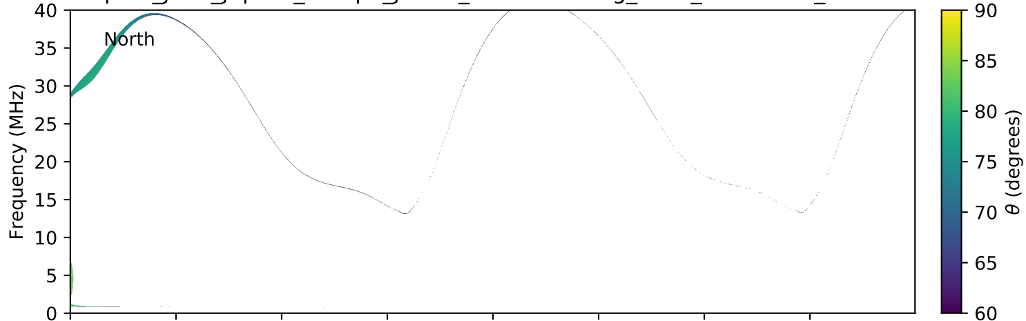
expres_juno_jupiter_europa_jrm09_lossc-wid1deg_3kev_20160520_v01.cdf
