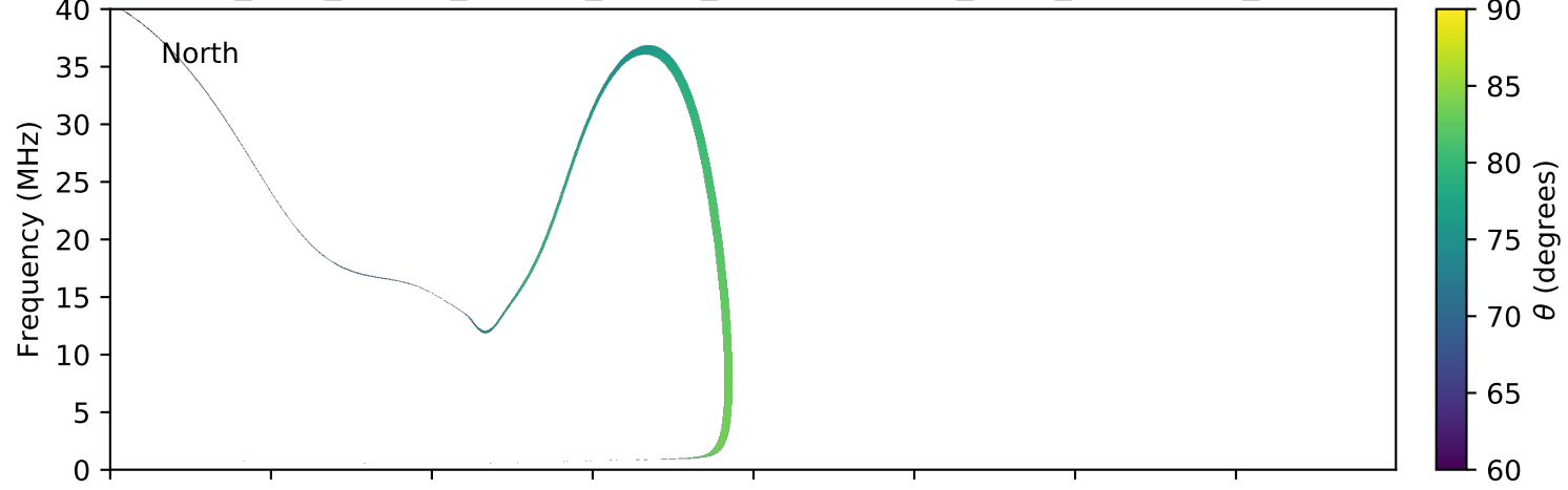
expres_juno_jupiter_europa_jrm09_lossc-wid1deg_3kev_20160507_v01.cdf
