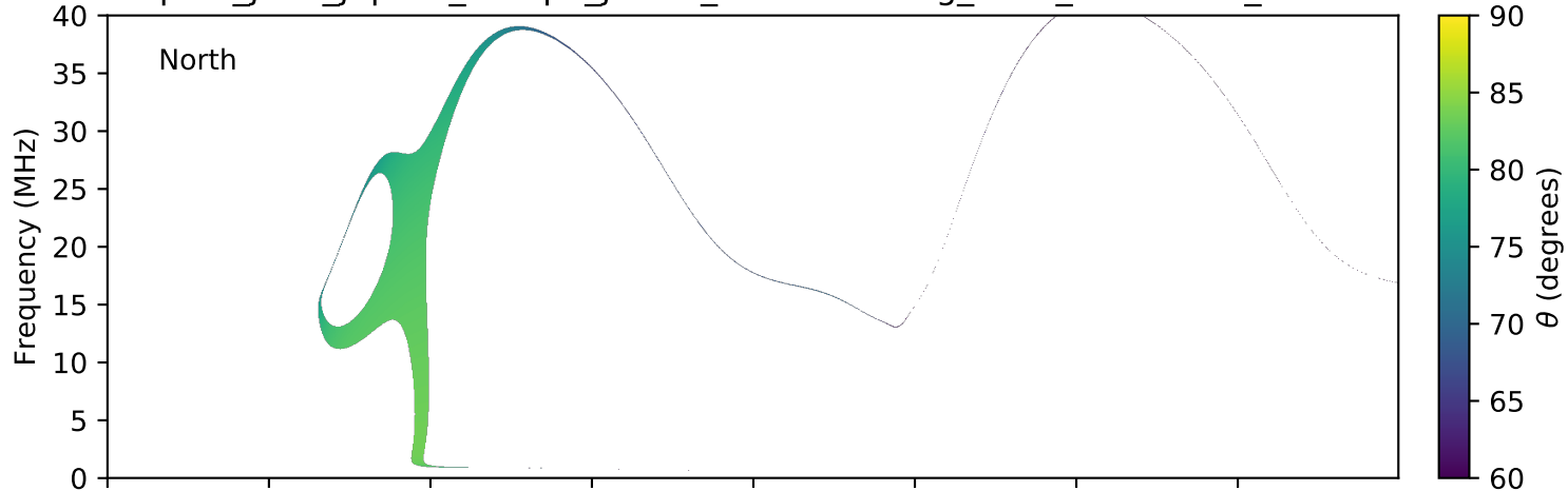
expres_juno_jupiter_europa_jrm09_lossc-wid1deg_3kev_20160502_v01.cdf
