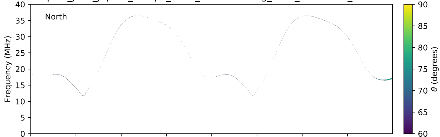
expres_juno_jupiter_europa_isaac_lossc-wid1deg_3kev_20160531_v01.cdf
