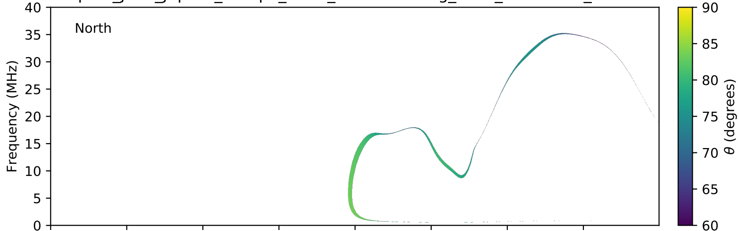
expres_juno_jupiter_europa_isaac_lossc-wid1deg_3kev_20160530_v01.cdf
