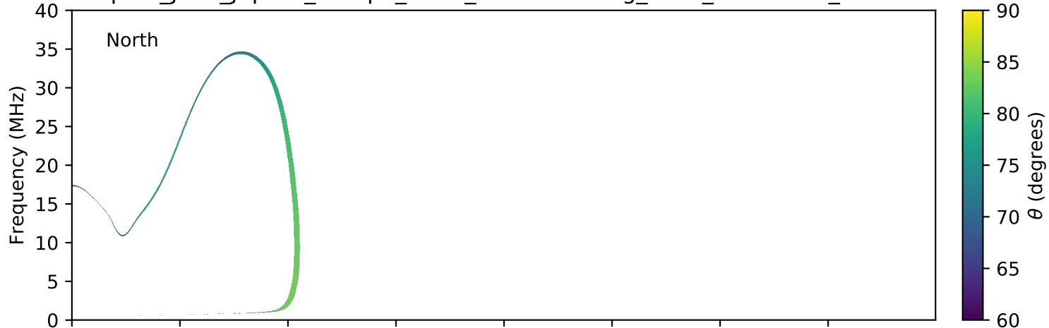
expres_juno_jupiter_europa_isaac_lossc-wid1deg_3kev_20160525_v01.cdf
