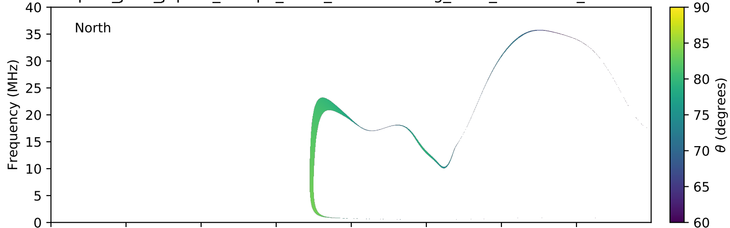
expres_juno_jupiter_europa_isaac_lossc-wid1deg_3kev_20160523_v01.cdf
