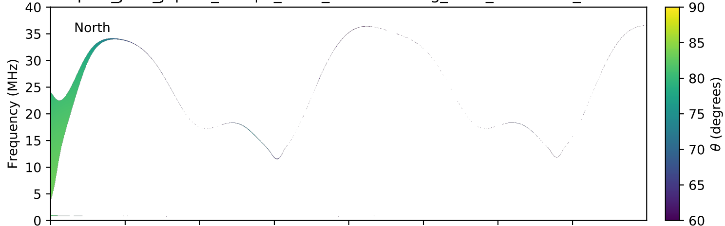
expres_juno_jupiter_europa_isaac_lossc-wid1deg_3kev_20160520_v01.cdf
