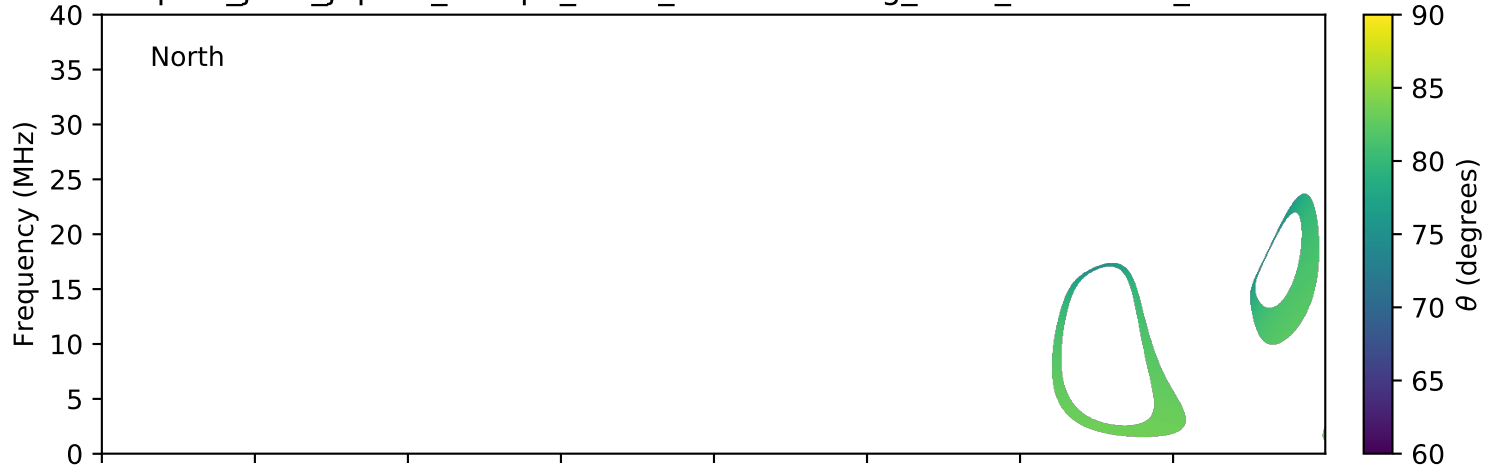
expres_juno_jupiter_europa_isaac_lossc-wid1deg_3kev_20160519_v01.cdf
