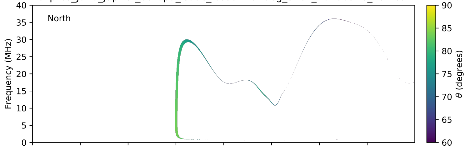
expres_juno_jupiter_europa_isaac_lossc-wid1deg_3kev_20160516_v01.cdf
