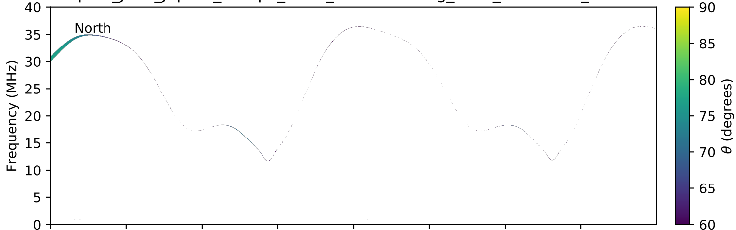
expres_juno_jupiter_europa_isaac_lossc-wid1deg_3kev_20160513_v01.cdf
