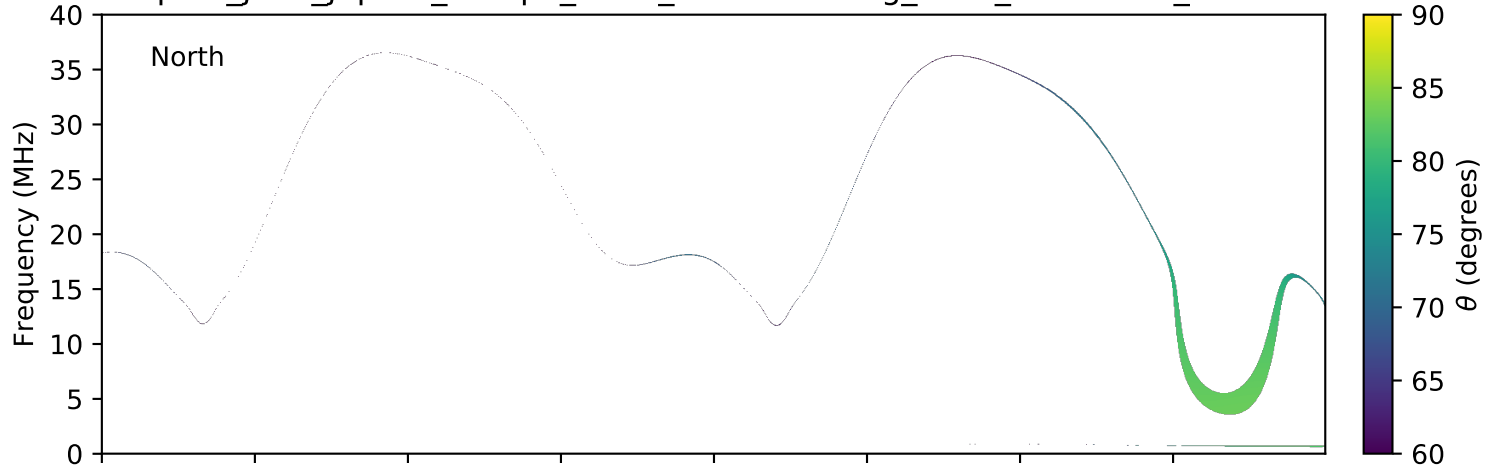
expres_juno_jupiter_europa_isaac_lossc-wid1deg_3kev_20160510_v01.cdf
