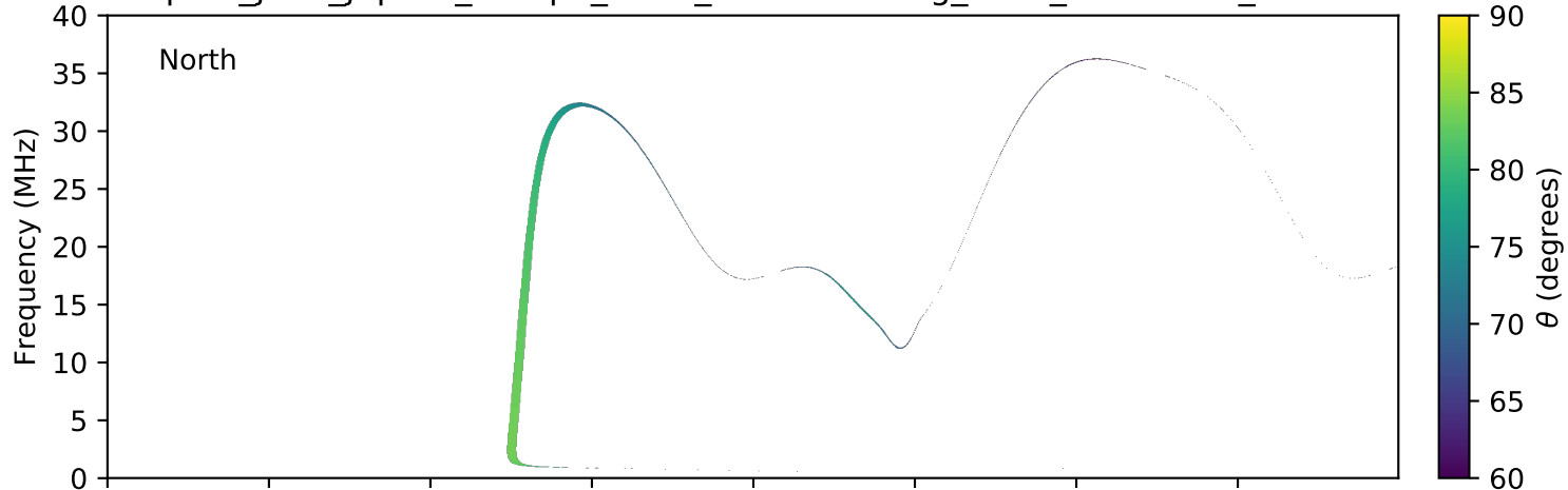
expres_juno_jupiter_europa_isaac_lossc-wid1deg_3kev_20160509_v01.cdf
