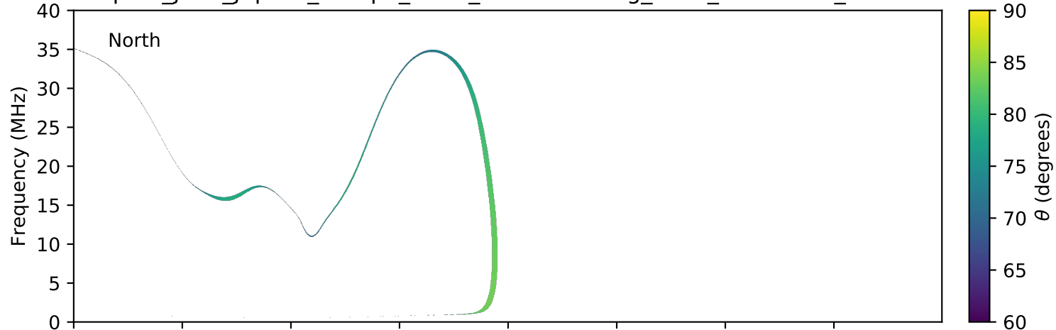
expres_juno_jupiter_europa_isaac_lossc-wid1deg_3kev_20160507_v01.cdf
