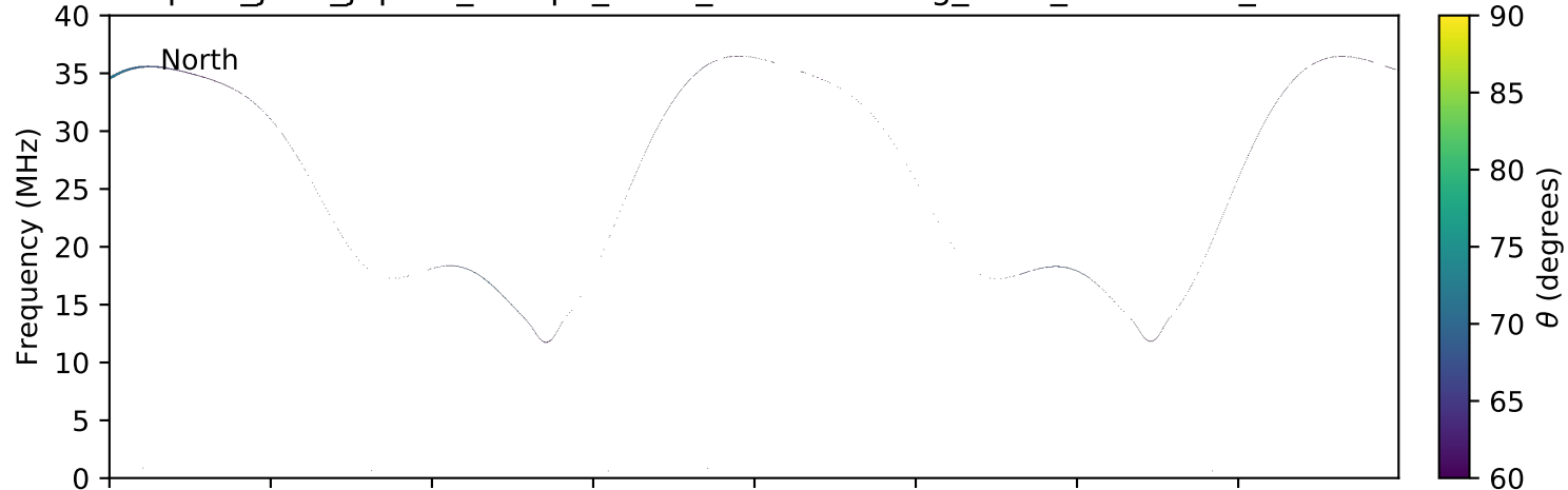
expres_juno_jupiter_europa_isaac_lossc-wid1deg_3kev_20160506_v01.cdf
