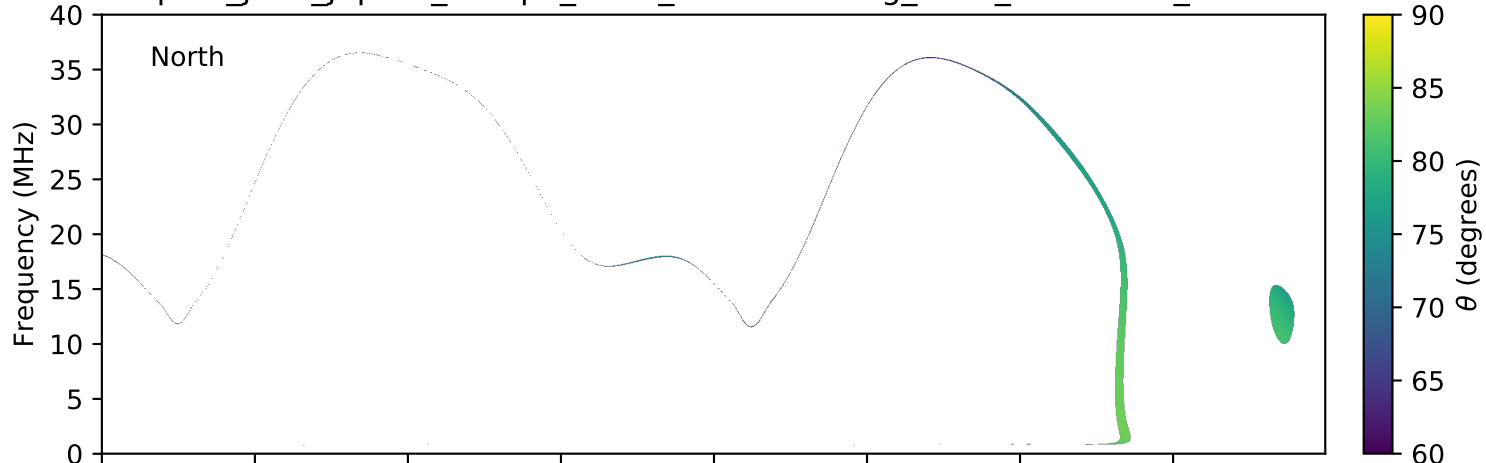
expres_juno_jupiter_europa_isaac_lossc-wid1deg_3kev_20160503_v01.cdf
