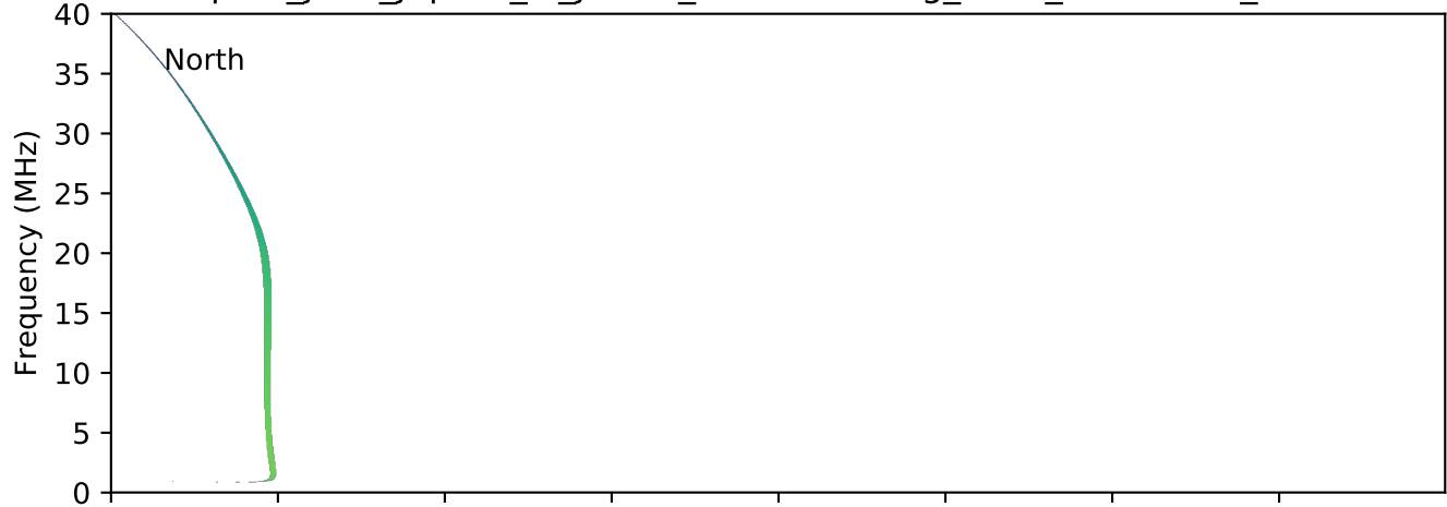
expres_juno_jupiter_io_jrm09_lossc-wid1deg_3kev_20160430_v01.cdf
