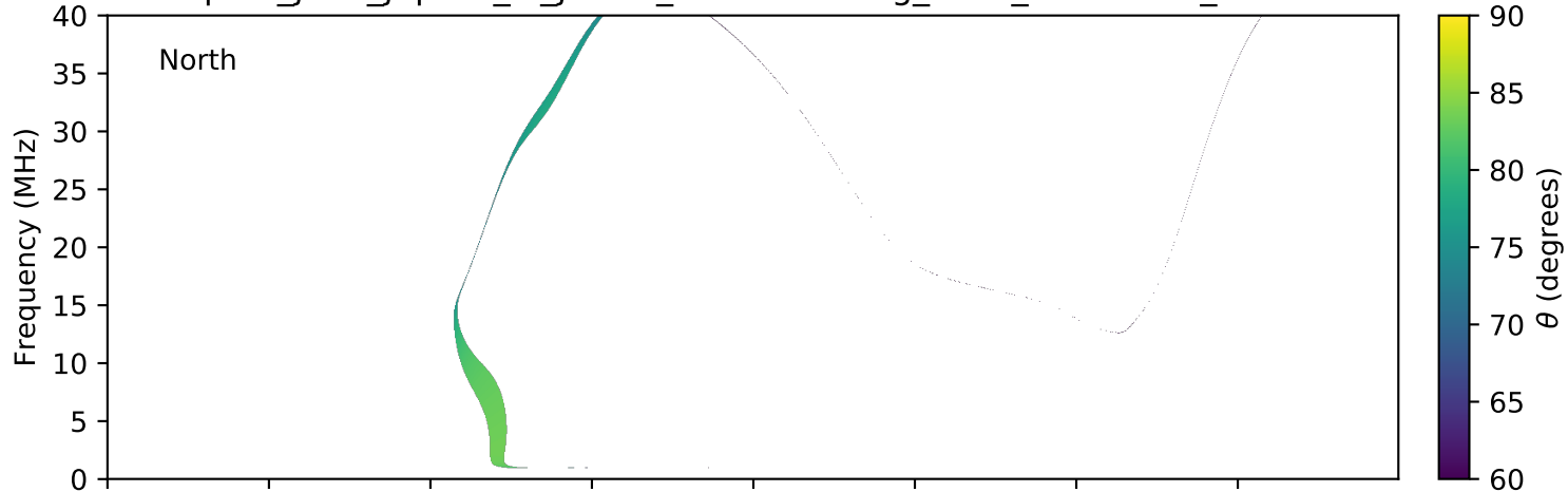
expres_juno_jupiter_io_jrm09_lossc-wid1deg_3kev_20160429_v01.cdf
