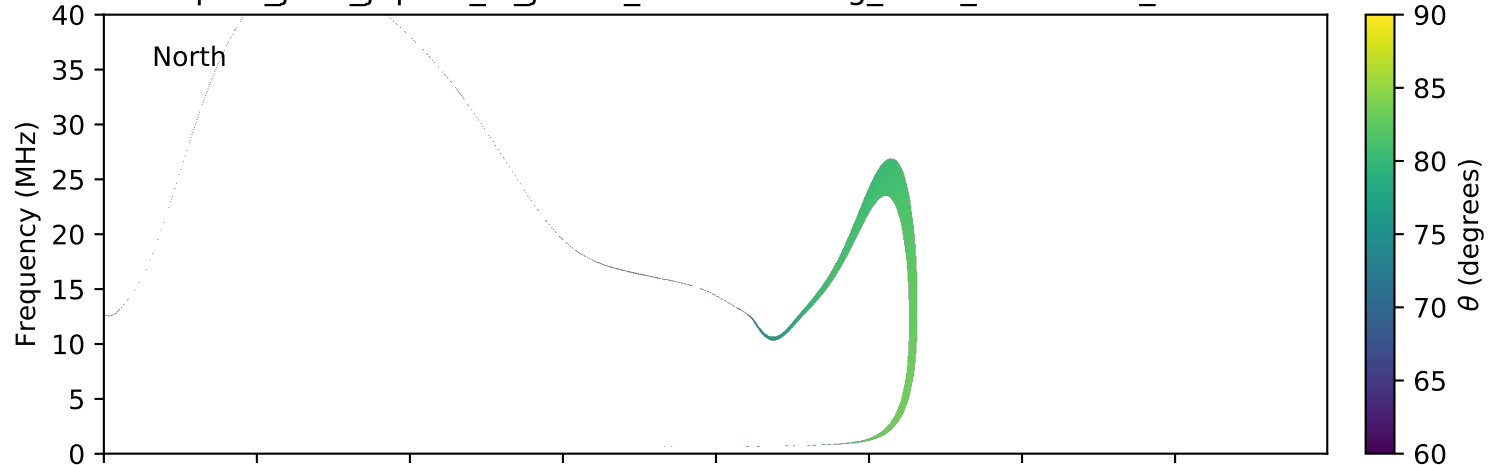
expres_juno_jupiter_io_jrm09_lossc-wid1deg_3kev_20160426_v01.cdf
