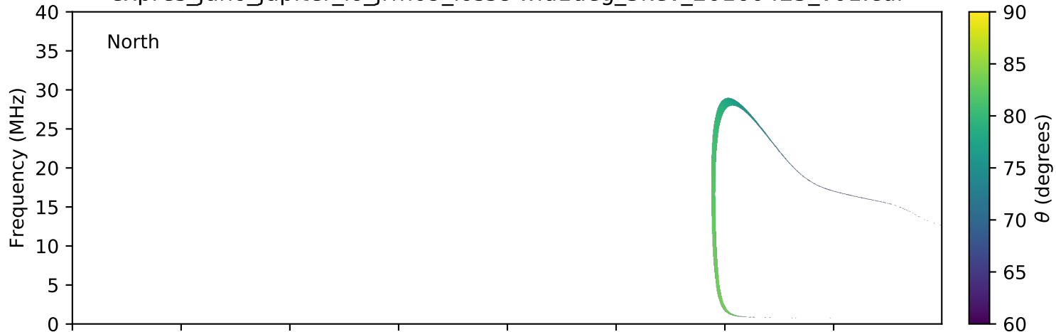
expres_juno_jupiter_io_jrm09_lossc-wid1deg_3kev_20160425_v01.cdf
