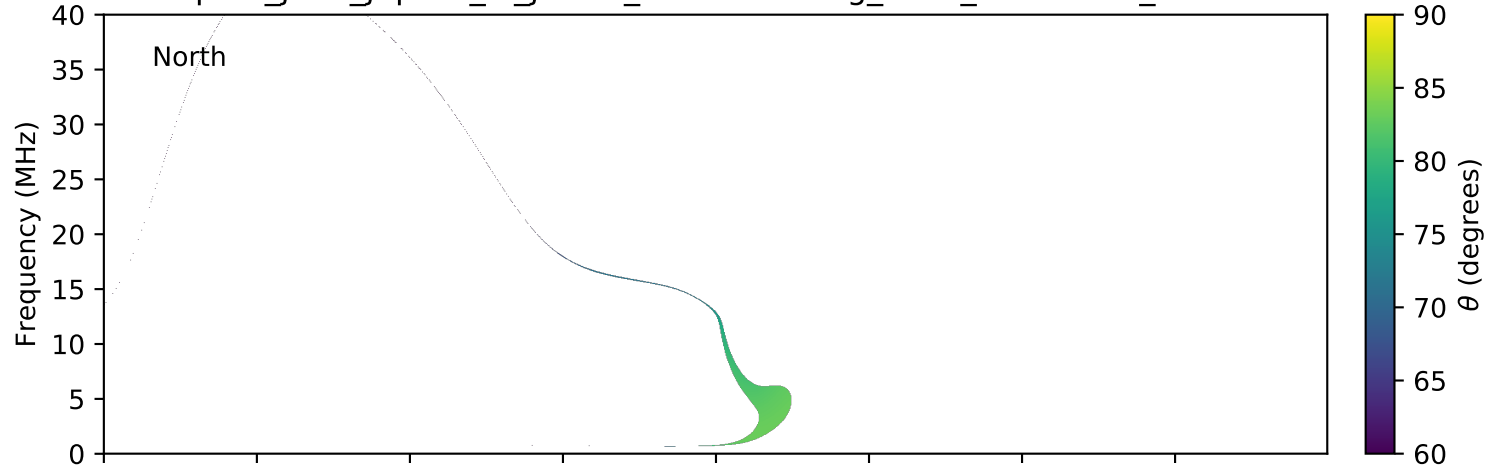
expres_juno_jupiter_io_jrm09_lossc-wid1deg_3kev_20160419_v01.cdf
