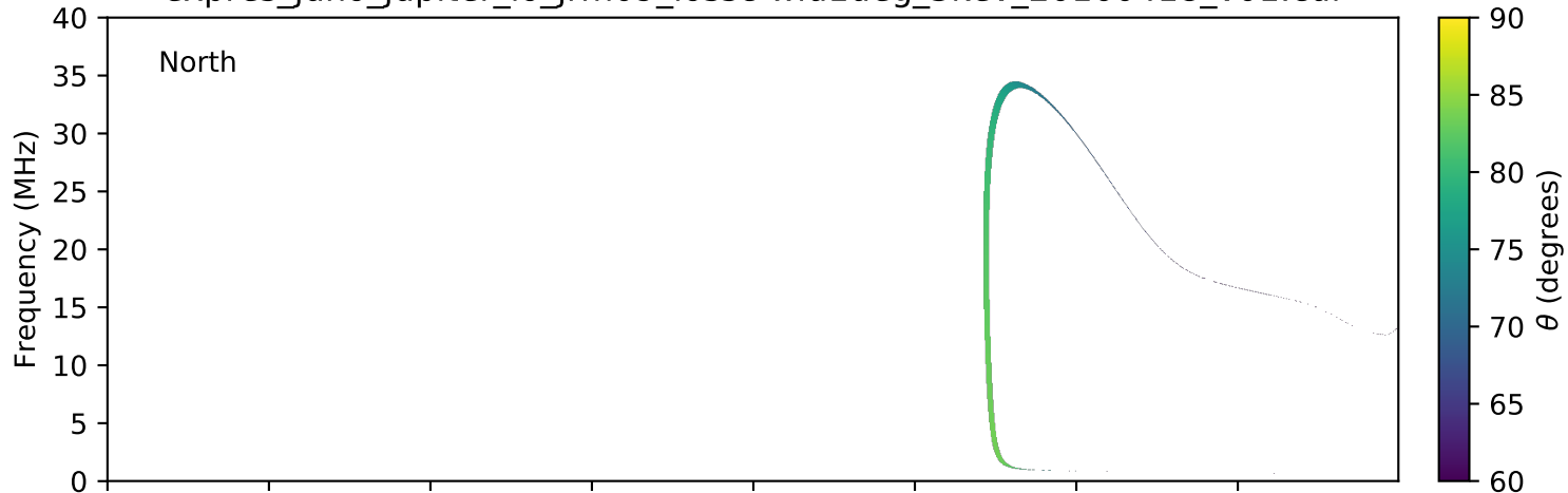
expres_juno_jupiter_io_jrm09_lossc-wid1deg_3kev_20160418_v01.cdf
