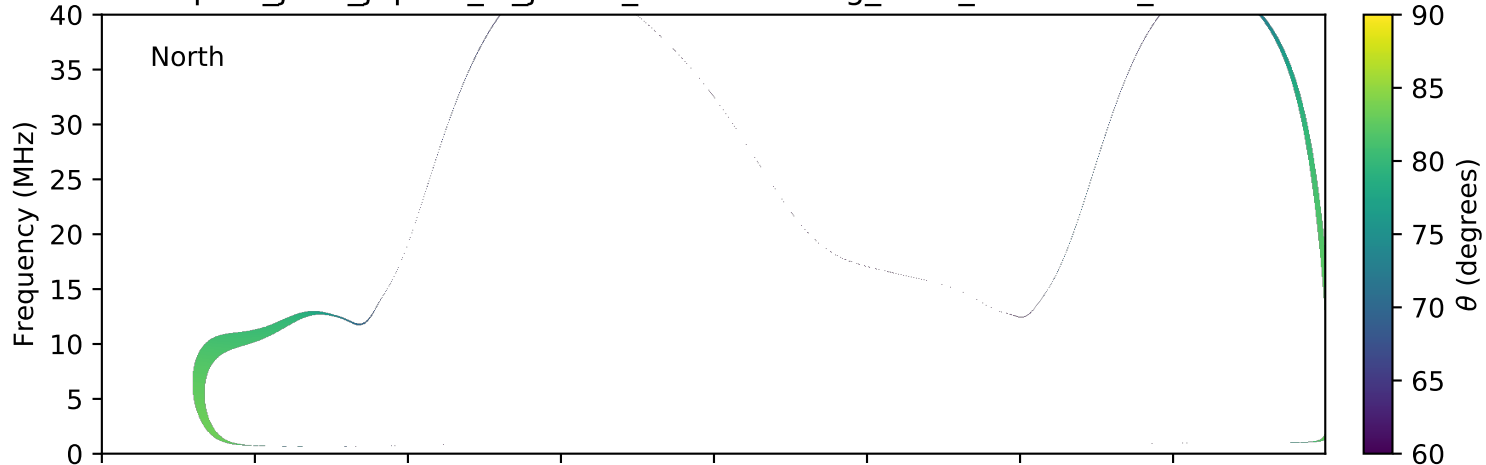
expres_juno_jupiter_io_jrm09_lossc-wid1deg_3kev_20160415_v01.cdf
