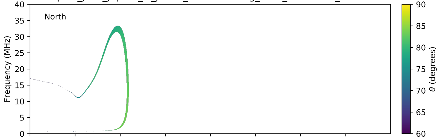
expres_juno_jupiter_io_jrm09_lossc-wid1deg_3kev_20160414_v01.cdf
