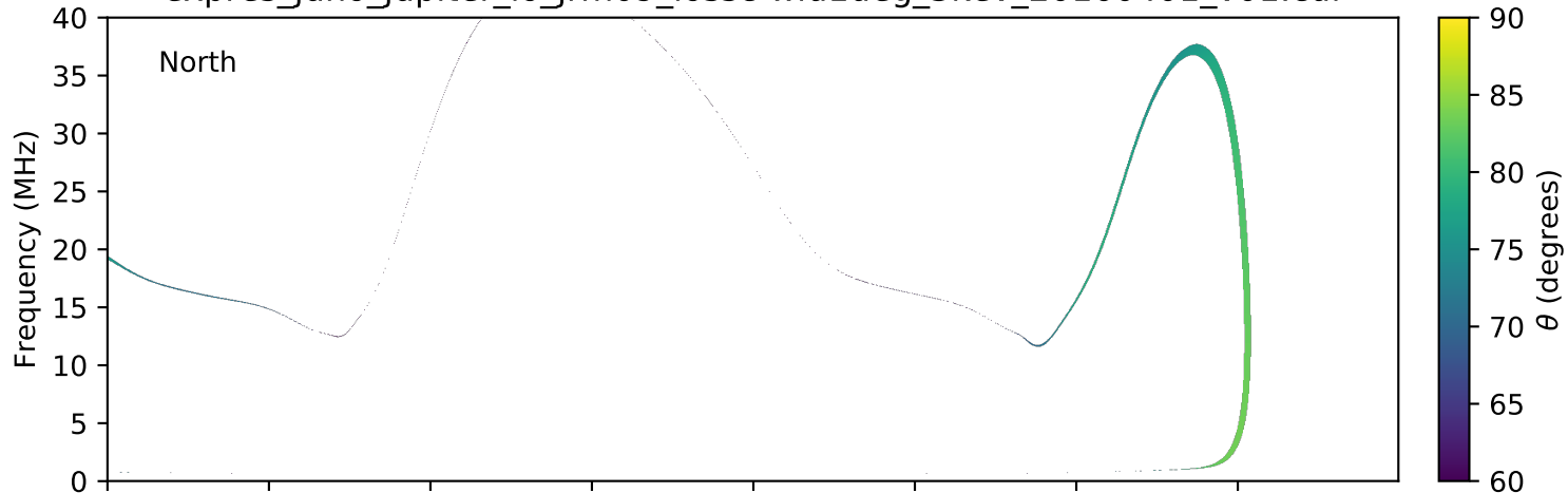
expres_juno_jupiter_io_jrm09_lossc-wid1deg_3kev_20160401_v01.cdf
