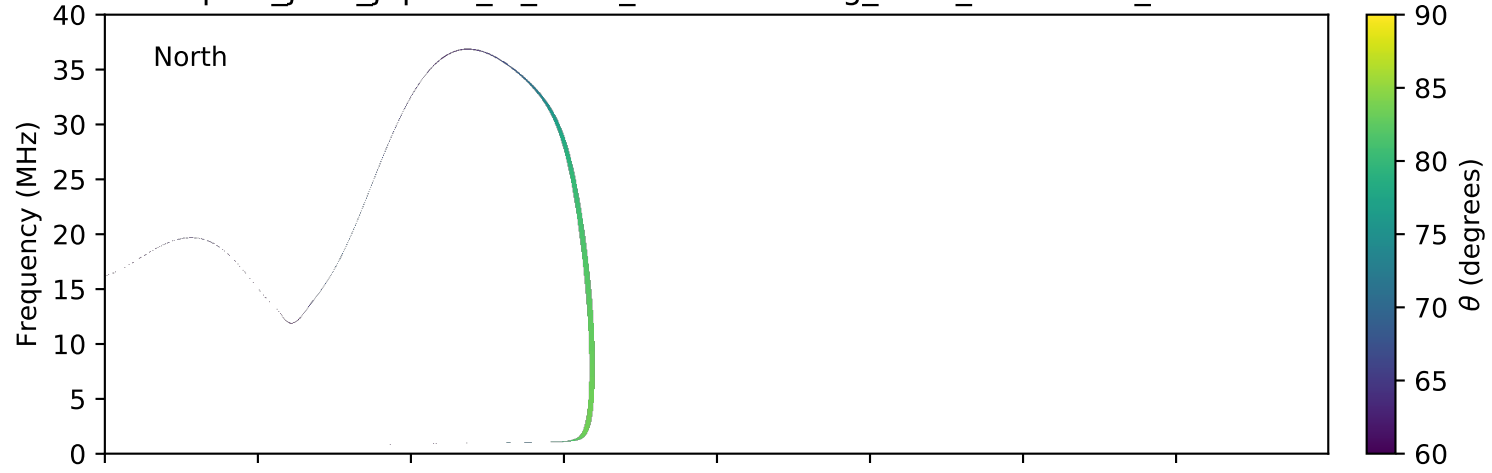
expres_juno_jupiter_io_isaac_lossc-wid1deg_3kev_20160428_v01.cdf
