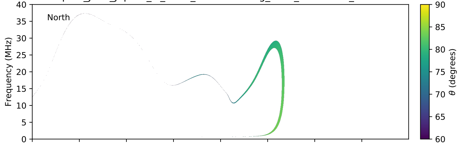
expres_juno_jupiter_io_isaac_lossc-wid1deg_3kev_20160426_v01.cdf
