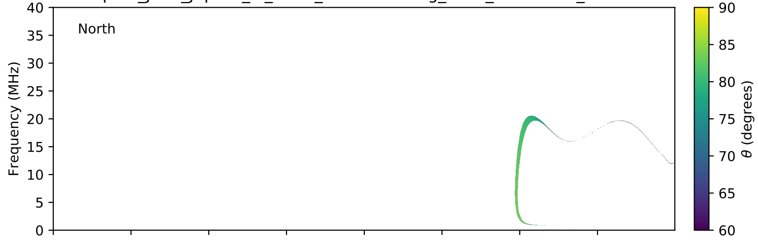
expres_juno_jupiter_io_isaac_lossc-wid1deg_3kev_20160425_v01.cdf
