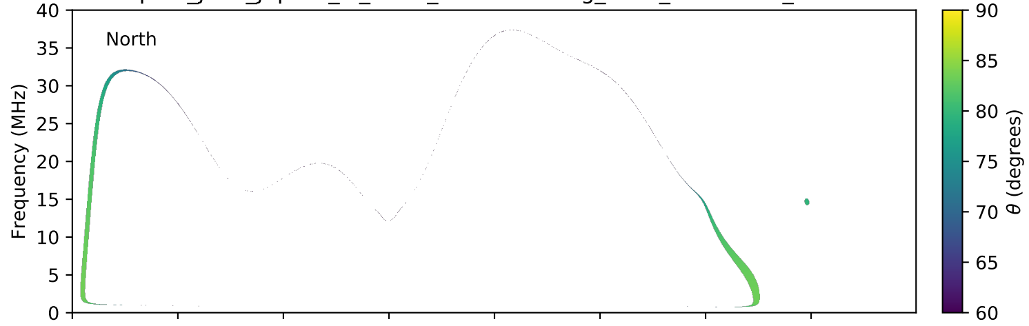
expres_juno_jupiter_io_isaac_lossc-wid1deg_3kev_20160424_v01.cdf
