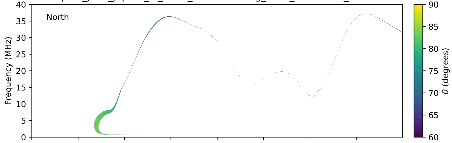
expres_juno_jupiter_io_isaac_lossc-wid1deg_3kev_20160422_v01.cdf
