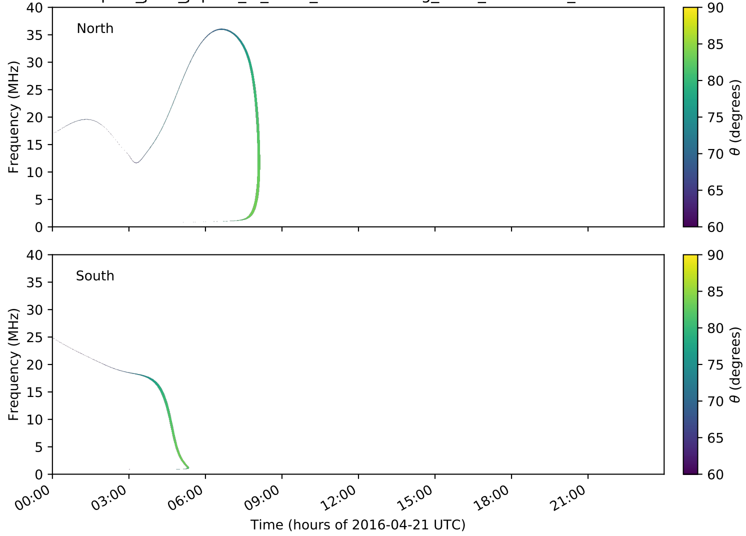
expres_juno_jupiter_io_isaac_lossc-wid1deg_3kev_20160421_v01.cdf
