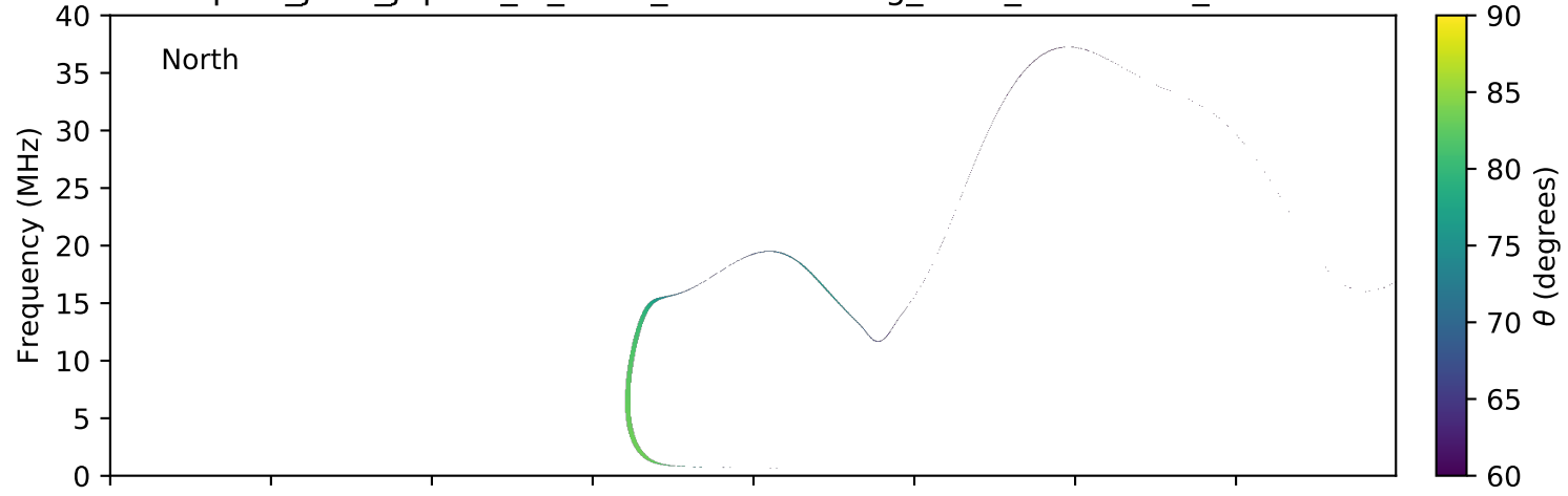
expres_juno_jupiter_io_isaac_lossc-wid1deg_3kev_20160420_v01.cdf
