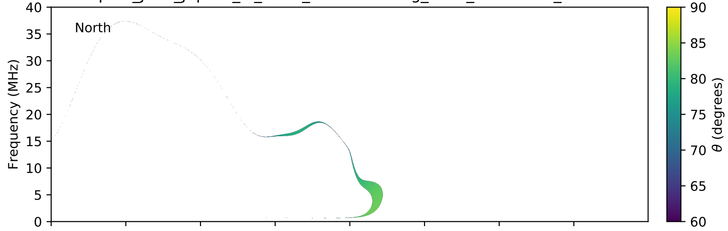
expres_juno_jupiter_io_isaac_lossc-wid1deg_3kev_20160419_v01.cdf
