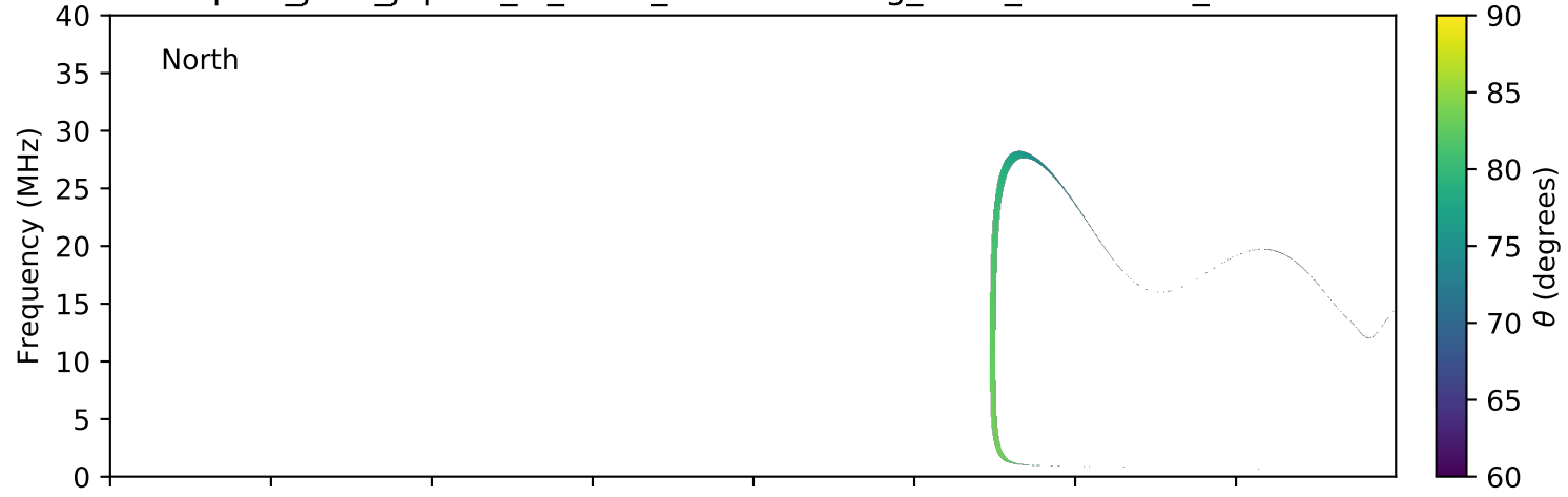
expres_juno_jupiter_io_isaac_lossc-wid1deg_3kev_20160418_v01.cdf
