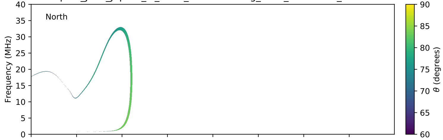
expres_juno_jupiter_io_isaac_lossc-wid1deg_3kev_20160414_v01.cdf
