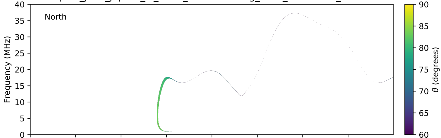
expres_juno_jupiter_io_isaac_lossc-wid1deg_3kev_20160413_v01.cdf
